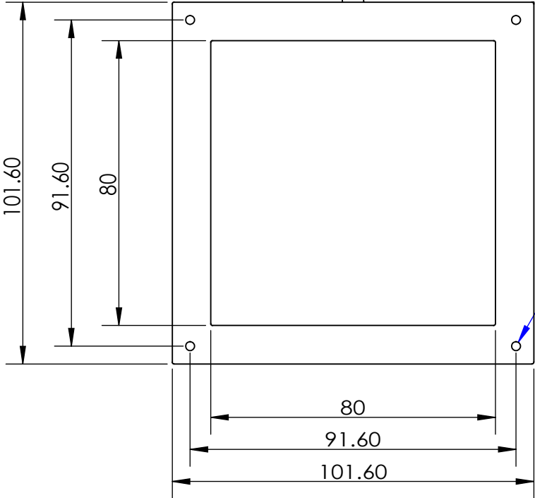
EMITTING AREA
