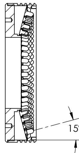
SECTION B-B SCALE 1 : 1.5
