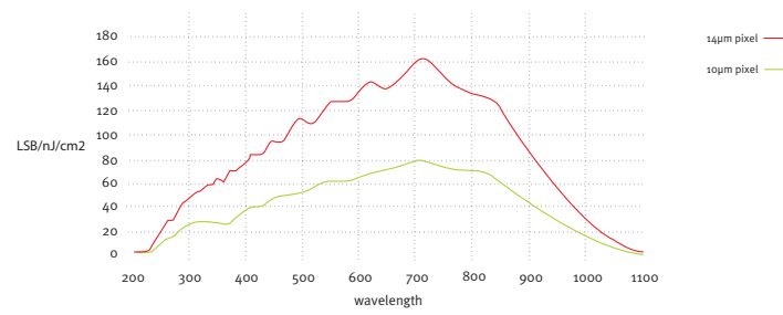
SPECTRAL RESPONSE DiViNA IN LSB 8BITS /NJ/CM 2
