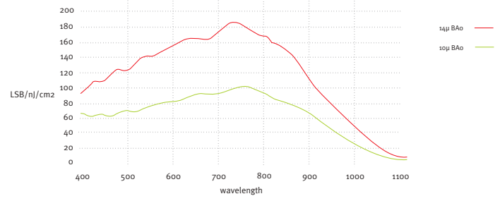
SPECTRAL RESPONSE ELiXA UC4/UC8 IN LSB 12BITS /NJ/CM 2 WITHOUT FILTER
