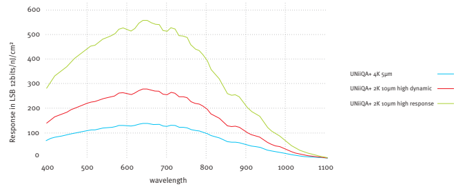
SPECTRAL RESPONSE UNiQA+ IN LSB 12BITS /NJ/CM 2
