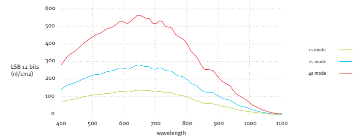
SPECTRAL RESPONSE AViVA2 EMX IN LSB 12BITS /NJ/CM 2
